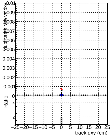
DOM mkFit TT base noSel DOM mkFit TT base 8iter noSel DOM mkFit TT retrainOldFiles v2 8iter2 noSel
