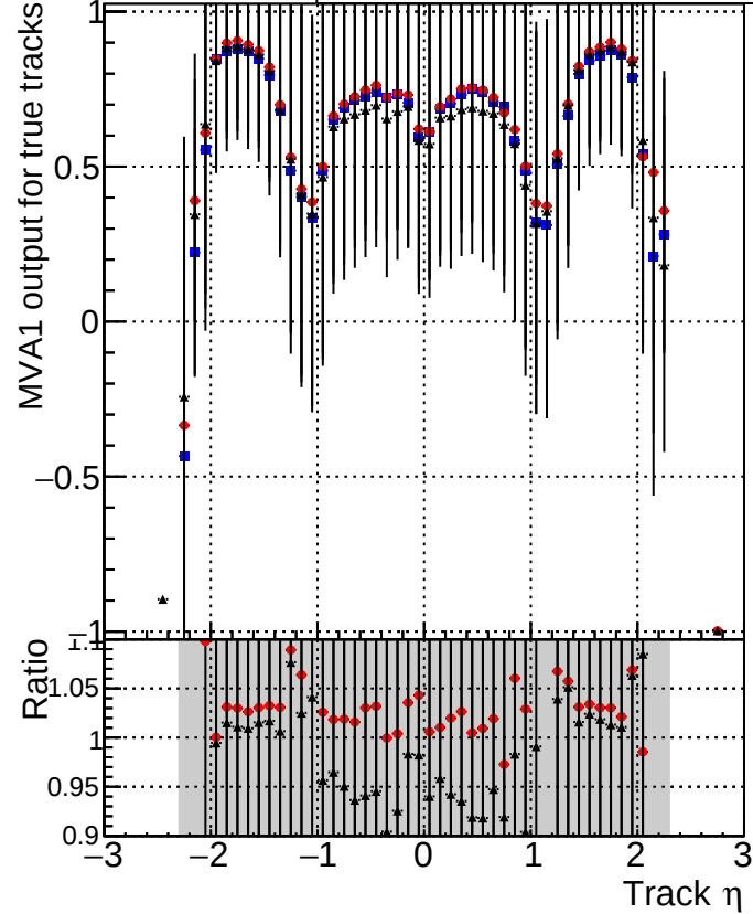
MVA1 of associated tracks (recoToSim) vs. track \eta Legend: DQM_mkFit_TT_base_noSel (blue squares) DQM_mkFit_TT_base_8iter_noSel (red diamonds) DQM_mkFit_TT_retrainOldFiles_v2_8iter2_noSel (black stars)
