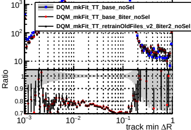
N of reconstructed tracks vs dR(track,jet)
