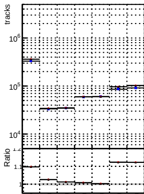
DOM mkFit TT base noSel DOM mkFit TT base 8iter noSel DOM mkFit TT retrainOldFiles v2 8iter2 noSel
