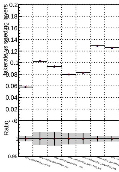
Fake rate vs. Legend: DOM mkFit TT base noSel base 8iter noSel DOM mkFit TT retrainOldFiles v2 8iter2 noSel
