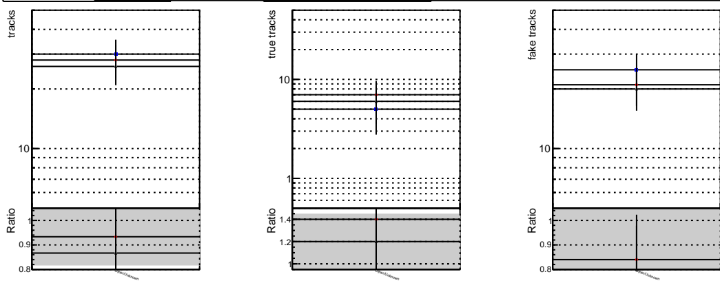
N of reco track vs. \chi^2 DQM mkFit base noSel DQM mkFit base 8iter noSel DQM mkFit retrainOldFiles v2 8iter2 noSel
