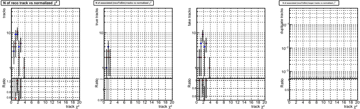
N of reco track vs. \chi^2 DQM mkFit base noSel DQM mkFit base 8iter noSel DQM mkFit retrainOldFiles v2 8iter2 noSel
