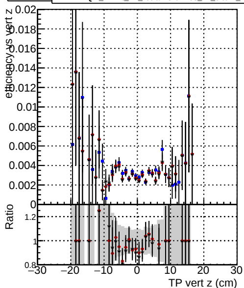
Efficiency —●— DQM_mkFit_TT_base_8iter_noSel —▲— DQM_mkFit_TT_retrainOldFiles_v2_8iter2_noSel
