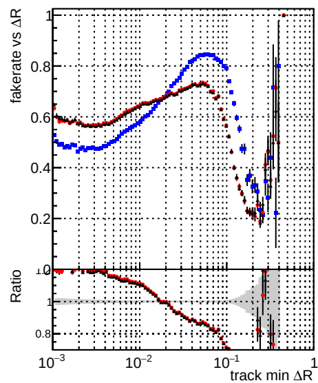
Legend for Fake rate vs dr, Duplicates Rate vs dr, Pileup rate vs dr: DQM mkFit TT base noSel (blue dots) DQM mkFit TT base 8iter noSel (red dots) DQM mkFit TT retrainOldFiles_v2_8iter2_noSel (black dots)
