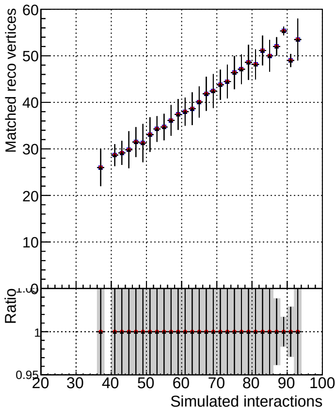
MatchedRecoVtx_vs_GenVtx
