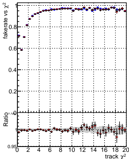
Fake rate vs. — DGM mkFit TT base noSel — DGM mkFit TT base 8iter noSel — DGM mkFit TT retrainOldFiles v2 8iter2 noSel
