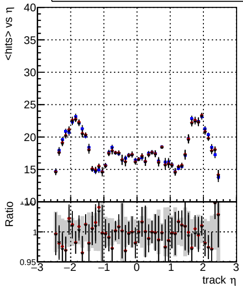
— DQM_mkFit_TT_base_noSel — DQM_mkFit_TT_base_8iter_noSel — DQM_mkFit_TT_retrainOldFiles_v2_8iter2_noSel mean hits
