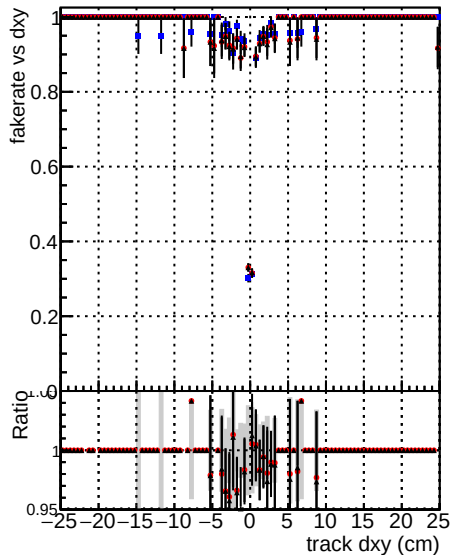
DOM mkFit TT base noSel DOM mkFit TT retrainOldFiles v2 8iter2 noSel
