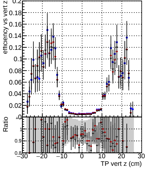
Efficiency vs. TP vert z (cm) — DQM_mkFit_TT_base_noSel — DQM_mkFit_TT_base_8iter_noSel — DQM_mkFit_TT_retrainOldFiles_v2_8iter2_noSel
