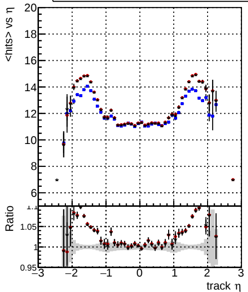
mean hits — DQM_mkFit_TT_base_noSel — DQM_mkFit_TT_base_8iter_noSel — DQM_mkFit_TT_retrainOldFiles_v2_8iter2_noSel
