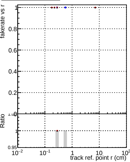
Fake rate vs v Legend: DQM_mkFit_TT_base_noSel (blue dots) DQM_mkFit_TT_base_8iter_noSel (red dots) DQM_mkFit_TT_retrainOldFiles_v2_8iter2_noSel (black dots)
