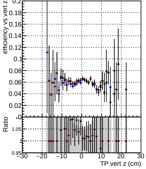
Efficiency vs TP vert z —●— DQM_mkFit_TT_base_noSel —●— DQM_mkFit_TT_base_8iter_noSel —●— DQM_mkFit_TT_retrainOldFiles_v2_8iter2_noSel
