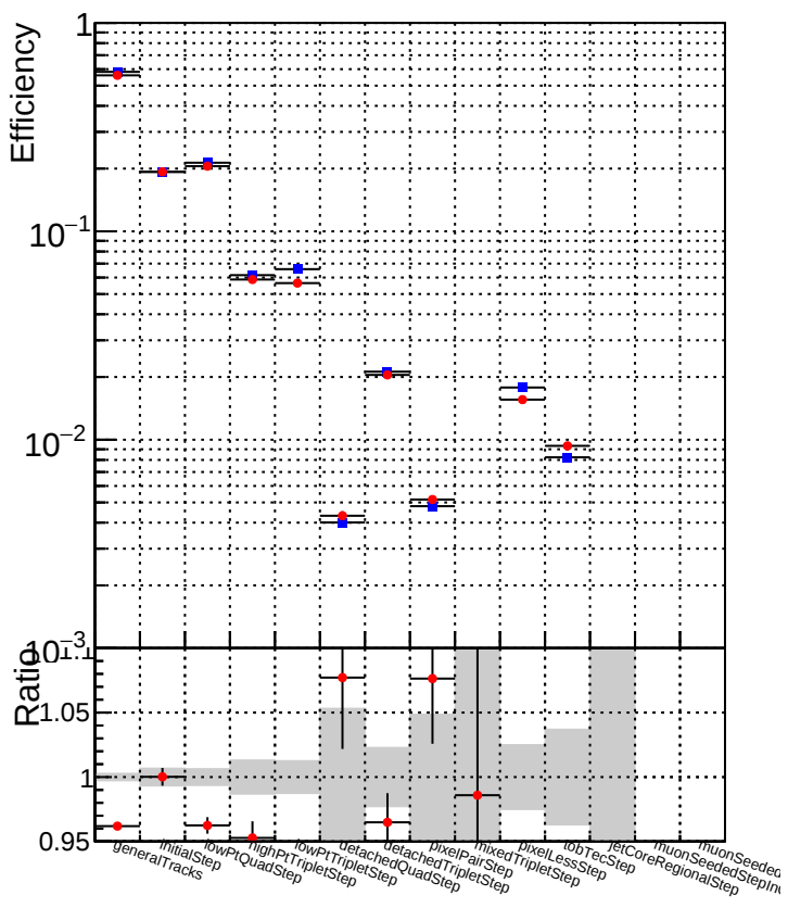
DQM_mkFit_TT_base_noSel DQM_mkFit_TT_retrainOldFiles_v2_8iter_noSel
