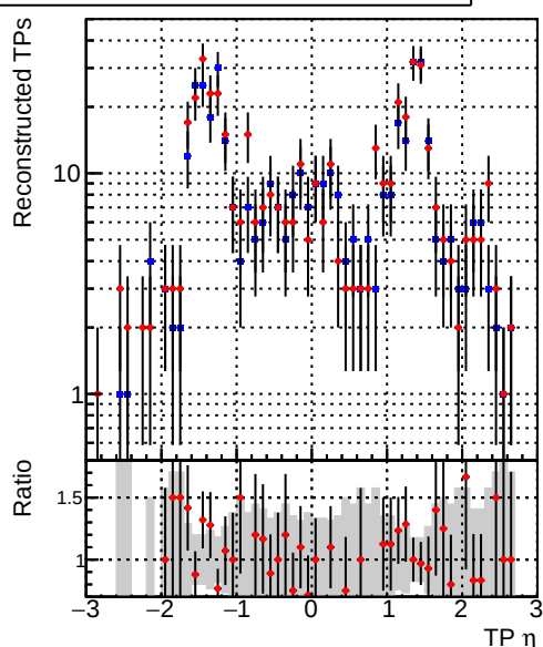
—●— DQM_mkFit_TT_base_noSel —●— DQM_mkFit_TT_retrainOldFiles_v2_8iter_noSel
