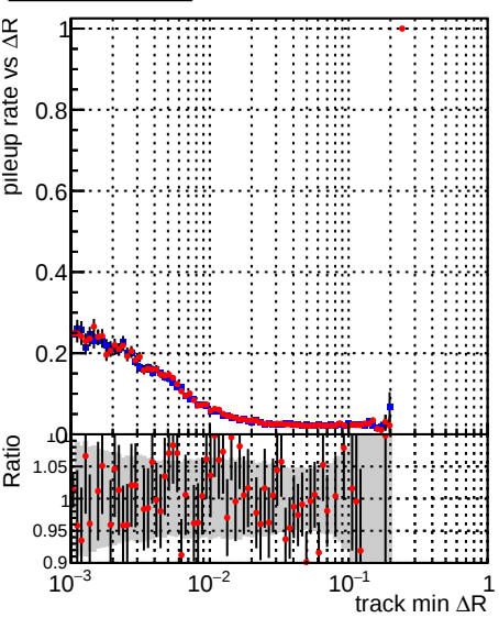
—•— DQM_mkFit_TT_base_noSel —•— DQM_mkFit_TT_retrainOldFiles_v2_8iter_noSel
