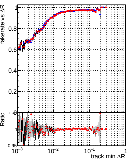
—•— DQM_mkFit_TT_base_noSel —•— DQM_mkFit_TT_retrainOldFiles_v2_8iter_noSel
