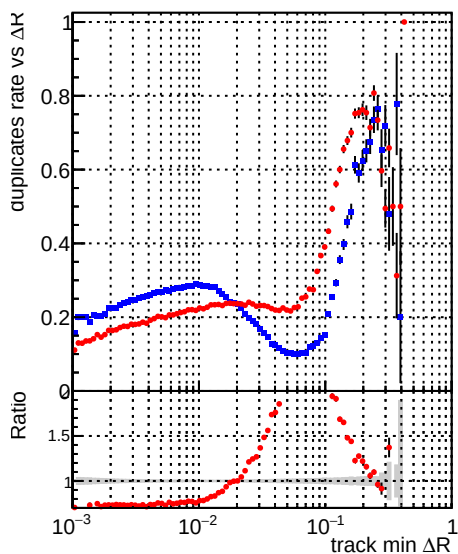
Legend: —●— DQM_mkFit_TT_base_noSel —●— DQM_mkFit_TT_retrainOldFiles_v2_8iter_noSel
