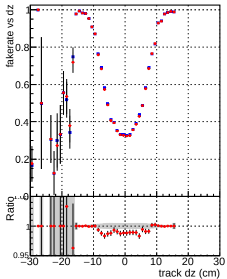
—●— DQM_mkFit_TT_base_noSel —●— DQM_mkFit_TT_retrainOldFiles_v2_8iter_noSel
