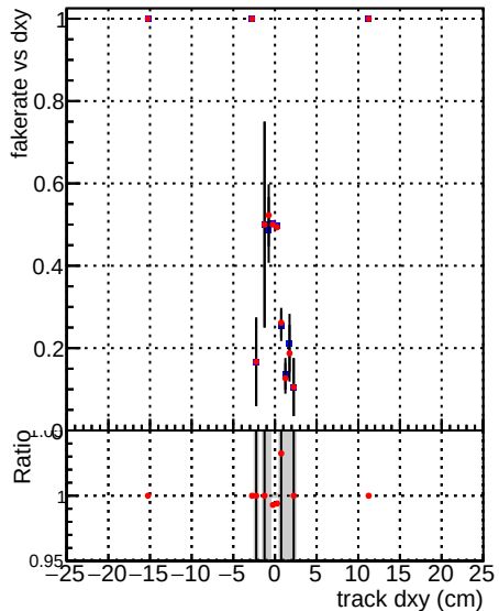
—●— DQM_mkFit_TT_base_noSel —●— DQM_mkFit_TT_retrainOldFiles_v2_8iter_noSel
