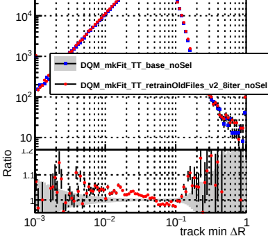
N of reconstructed tracks vs dR(track, jet)
