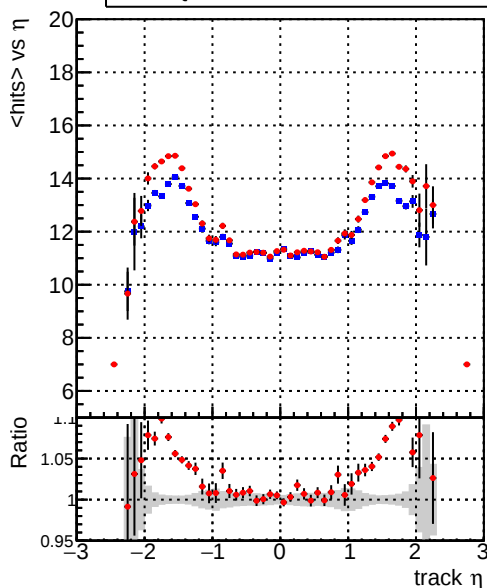
— DQM_mkFit_TT_base_noSel — DQM_mkFit_TT_retrainOldFiles_v2_8iter_noSel
