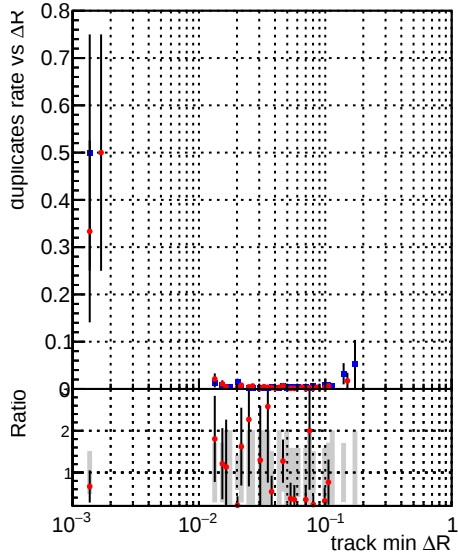
—•— DQM_mkFit_TT_base_noSel —•— DQM_mkFit_TT_retrainOldFiles_v2_8iter_noSel
