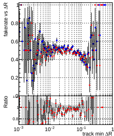
—•— DQM_mkFit_TT_base_noSel —•— DQM_mkFit_TT_retrainOldFiles_v2_8iter_noSel
