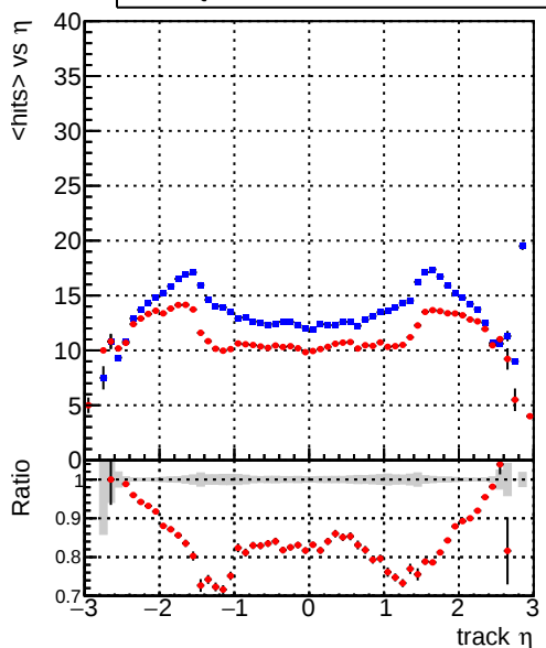
— DQM_mkFit_TT_base_noSel — DQM_mkFit_TT_retrainOldFiles_v2_8iter_noSel mean hits
