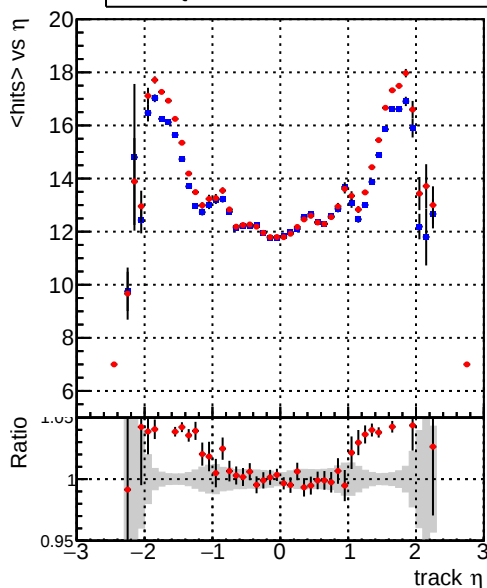
mean hits vs \eta — DQM_mkFit_TT_base_noSel — DQM_mkFit_TT_retrainOldFiles_v2_8iter_noSel
