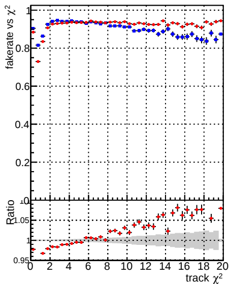
Fake rate vs. —●— DQM_mkFit_TT_base_noSel —●— DQM_mkFit_TT_retrainOldFiles_v2_8iter_noSel
