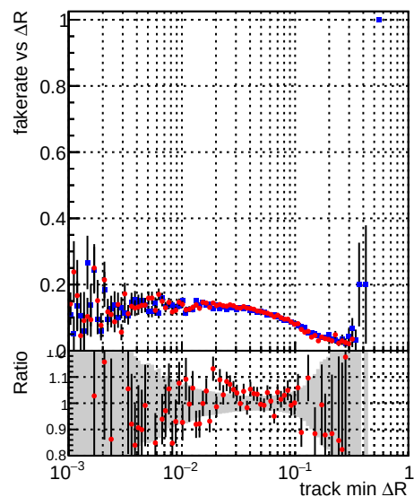
—•— DQM_mkFit_TT_base_noSel —•— DQM_mkFit_TT_retrainOldFiles_v2_8iter_noSel
