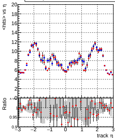
mean hit — DQM_mkFit_TT_base_noSel — DQM_mkFit_TT_retrainOldFiles_v2_8iter_noSel
