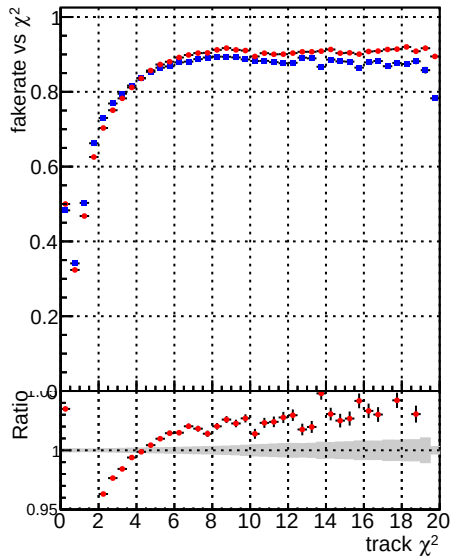
Fake rate vs. —■— DQM mkFit TT base_noSel —●— DQM mkFit TT retrainOldFiles_v2 8iter_noSel
