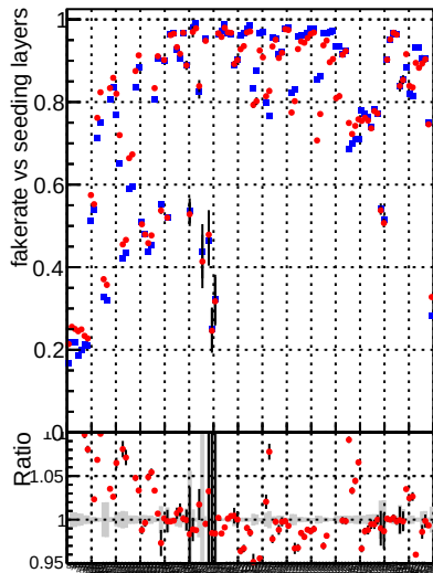
Fake rate vs. —■— DQM mkFit TT base_noSel —●— DQM mkFit TT retrainOldFiles_v2 8iter_noSel
