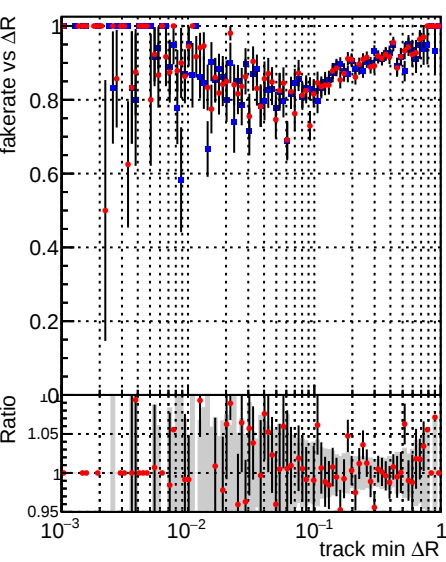
Legend: ■ DQM_mkFit_TT_base_noSel ● DQM_mkFit_TT_retrainOldFiles_v2_8iter_noSel
