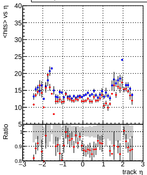
mean hits Legend: DQM_mkFit_TT_base_noSel (blue line), DQM_mkFit_TT_retrainOldFiles_v2_8iter_noSel (red line)
