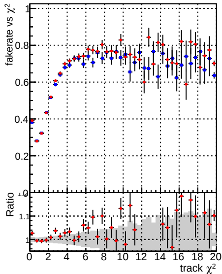
Fake rate vs. Legend: DQM_mkFit_TT_base_noSel (blue circles) DQM_mkFit_TT_retrainOldFiles_v2_8iter_noSel (red circles)
