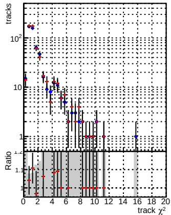
N of reco track vs. \chi^2 —●— DQM mkFit TT_base_noSel —●— DQM mkFit TT_retrainOldFiles_v2_8iter_noSel
