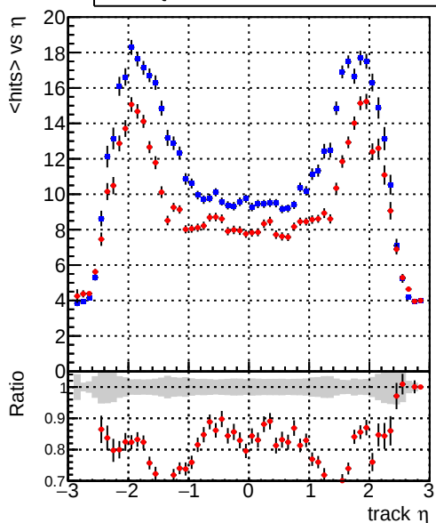
mean hits vs \eta Legend: DQM_mkFit_TT_base_noSel (blue line), DQM_mkFit_TT_retrainOldFiles_v2_8iter_noSel (red line)
