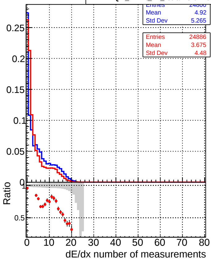
■ DQM_mkFit_TT_base_noSel ● DQM_mkFit_TT_retrainOldFiles_v2_8iter_noSel
