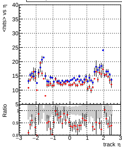
mean hits Legend: DQM_mkFit_TT_base_noSel (blue line), DQM_mkFit_TT_retrainOldFiles_v2_8iter_noSel (red line)
