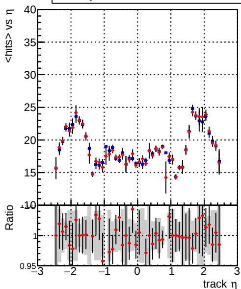
mean hits — DQM_mkFit_TT_base_noSel — DQM_mkFit_TT_retrainOldFiles_v2_8iter_noSel
