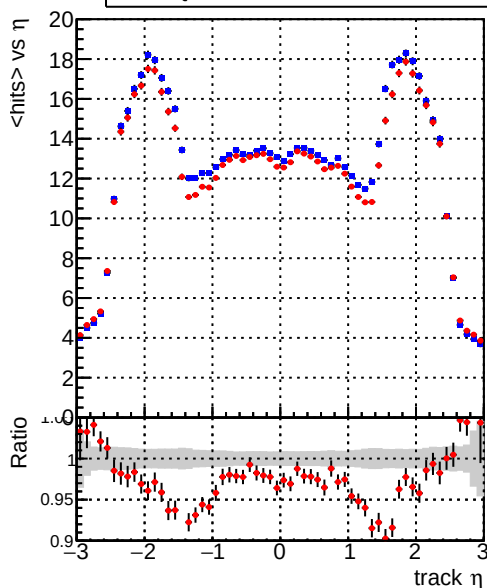
— DQM_mkFit_TT_base_noSel — DQM_mkFit_TT_retrainOldFiles_v2_8iter_noSel mean hits
