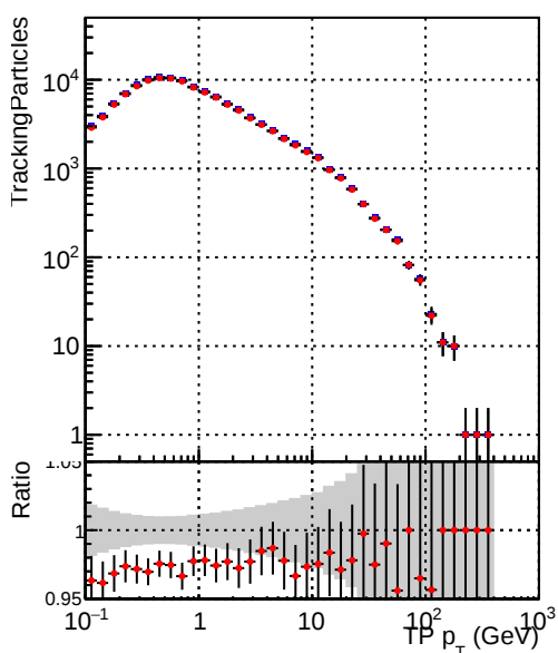
Legend: \blacksquare DQM_mkFit_TT_base_noSel \bullet DQM_mkFit_TT_retrainOldFiles_v2_8iter_noSel
