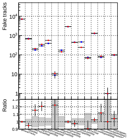
Number —●— DQM_mkFit_TT_retrainOldFiles_v2_8iter_noSel
