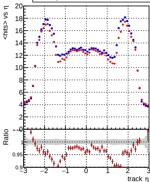
mean hit Legend: DQM_mkFit_TT_base_noSel (blue line), DQM_mkFit_TT_retrainOldFiles_v2_8iter_noSel (red line)
