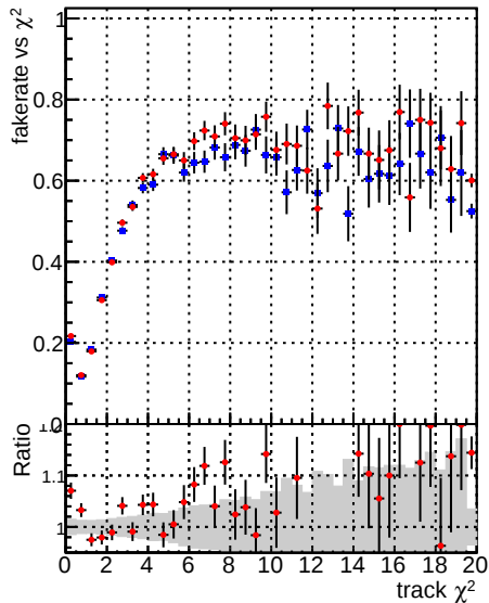
Fake rate vs. Legend: DQM_mkFit_TT_base_noSel (blue diamonds) DQM_mkFit_TT_retrainOldFiles_v2_8iter_noSel (red diamonds)
