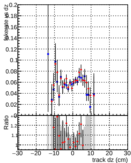
—●— DQM_mkFit_TT_base_noSel —●— DQM_mkFit_TT_retrainOldFiles_v2_8iter_noSel
