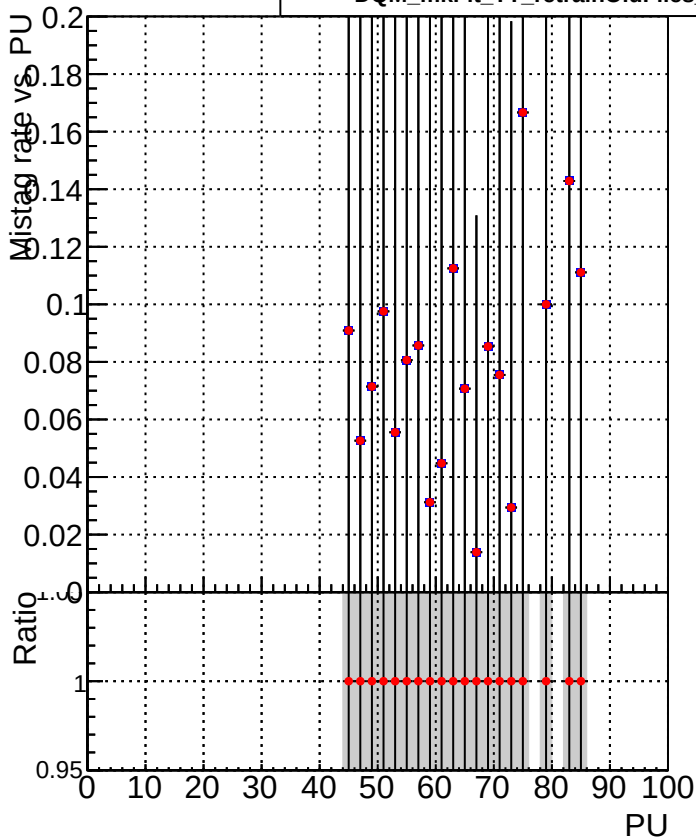
—•— DQM_mkFit_TT_base_noSel —•— DQM_mkFit_TT_retrainOldFiles_v2_8iter_noSel
