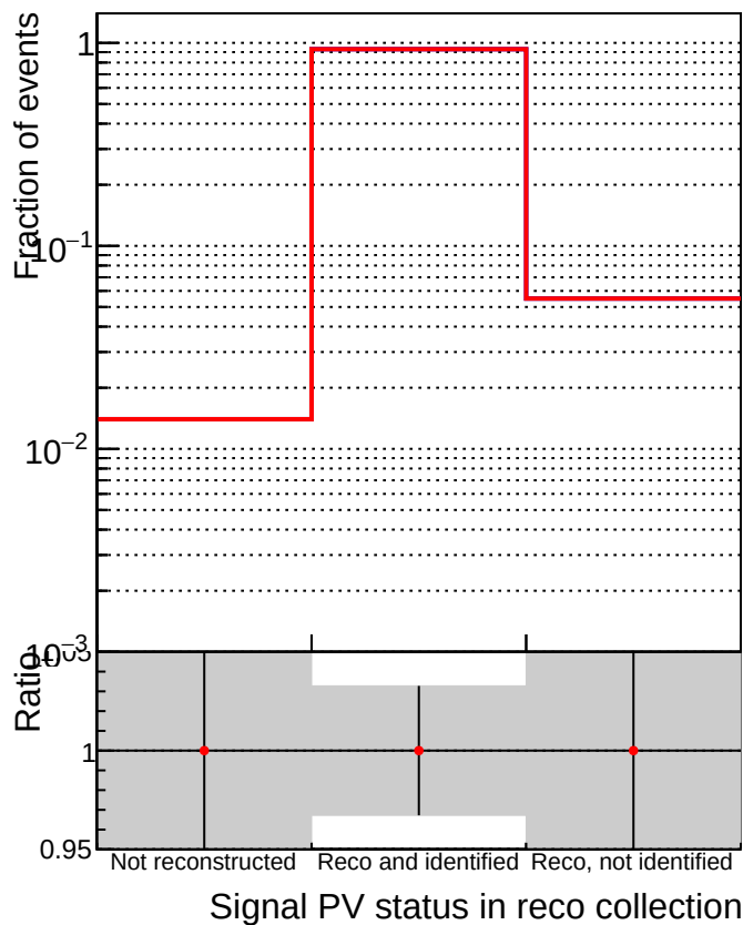
—•— DQM_mkFit_TT_base_noSel —•— DQM_mkFit_TT_retrainOldFiles_v2_8iter_noSel
