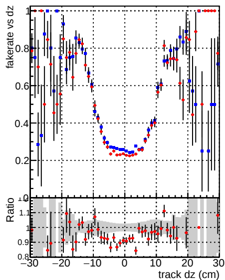
Fake rate vs dz —●— DQM_mkFit_TT_base_noSel —●— DQM_mkFit_TT_retrainOldFiles_v2_8iter_noSel
