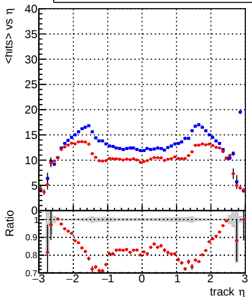
mean hits vs \eta Legend: DQM_mkFit_TT_base_noSel (blue line), DQM_mkFit_TT_retrainOldFiles_v2_8iter_noSel (red line)
