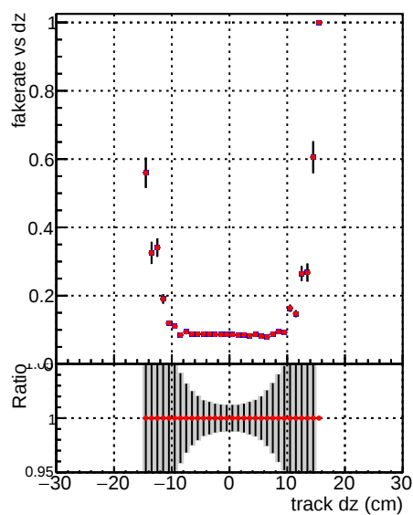
Fake rate vs dz — DQM_mkFit_TT_base_noSel — DQM_mkFit_TT_retrainOldFiles_v2_8iter_noSel
