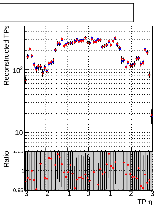
N of simulated tracks vs \eta
