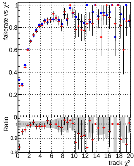
Fake rate vs. \chi^2 for various track selection cuts
